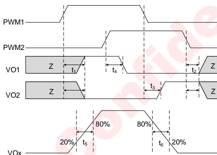
Figure 4 Input and Output Timing for AW8637
